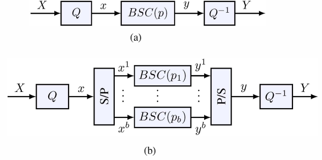
Fig. 1. Virtual correlation channel models for continuous-valued sources ( X and Y ) in the binary domain (a) Current model. (b) New model for b -bit scalar quantizer. x^1 to x^b are b subsequences of x that contain data belonging to the different bit-planes.
